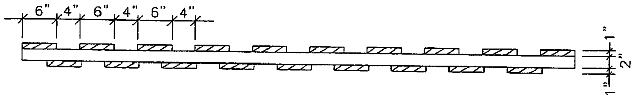
PLAN VIEW (2"x4"Horizontal Rail on Flat)
