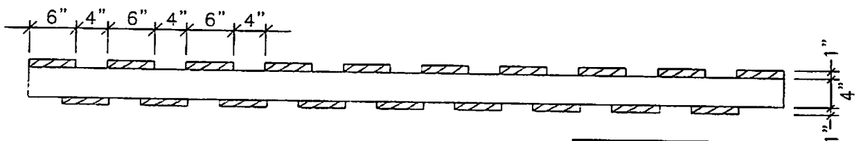
PLAN VIEW (2"x4"Horizontal Rail on Flat)
